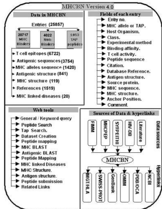
Figure 1 Detailed architecture of MHCBN database.
