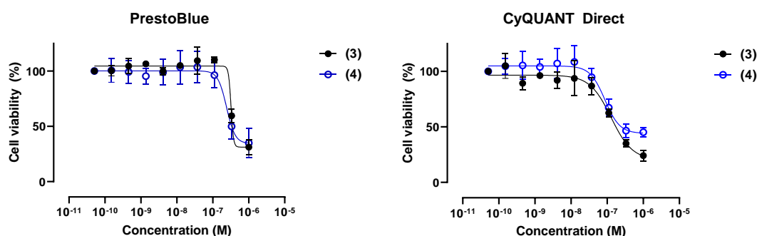
Figure 4. Percent viability of BxPC-3 human PDAC cells following 3 day exposure to trichoderin A (3) and its simplified analogue (4), as judged by the PrestoBlue™ and CyQUANT™ Direct assays.
