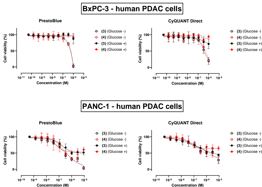
Figure 5. Comparative percent viability of BxPC-3 and PANC-1 human PDAC cells cultured under 'low glucose' (Glucose −) and 'normal glucose' (Glucose +) conditions following a 24 h exposure to trichoderin A (3) and its simplified analogue (4), as judged by the PrestoBlue™ and CyQUANT™ Direct assays.
