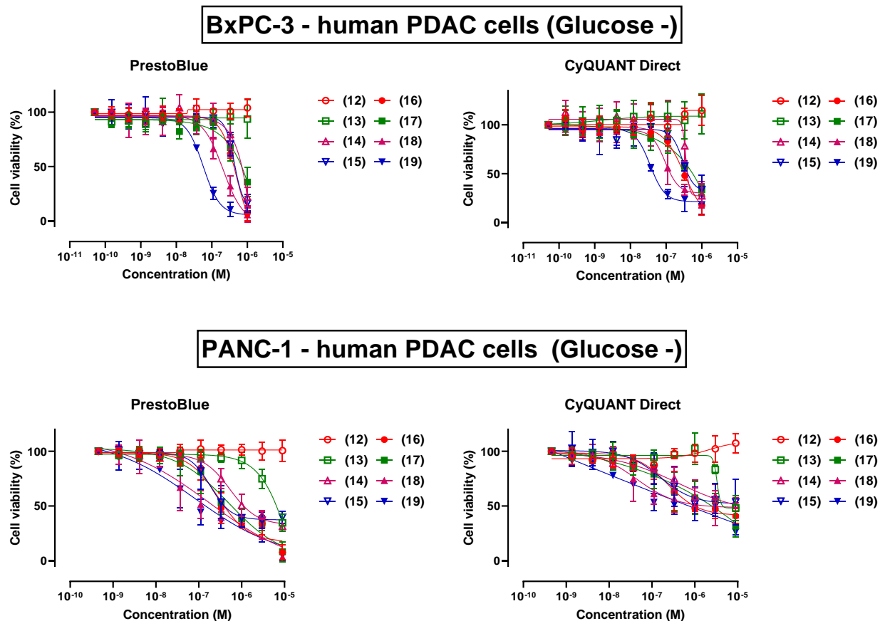
Figure 7. Comparative percent viability of BxPC-3 and PANC-1 cells cultured under ‘low glucose’ (Glucose –) following a 24 h exposure to trichoderin A analogues (12)–(19), as judged by the PrestoBlue™ and CyQUANT™ Direct assays.
