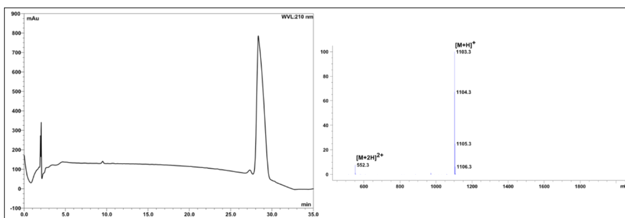
Scheme 1. Hybrid solid-/solution-phase synthesis of the simplified trichoderin A analogue (4).
