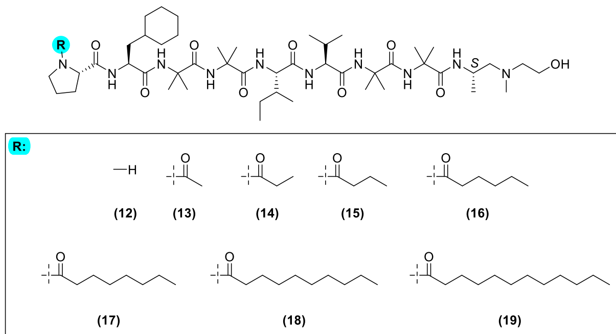
Figure 6. General structure of the simplified trichoderin A analogue (4). The N-terminus has been modified accordingly to generate analogues (12)–(19).
