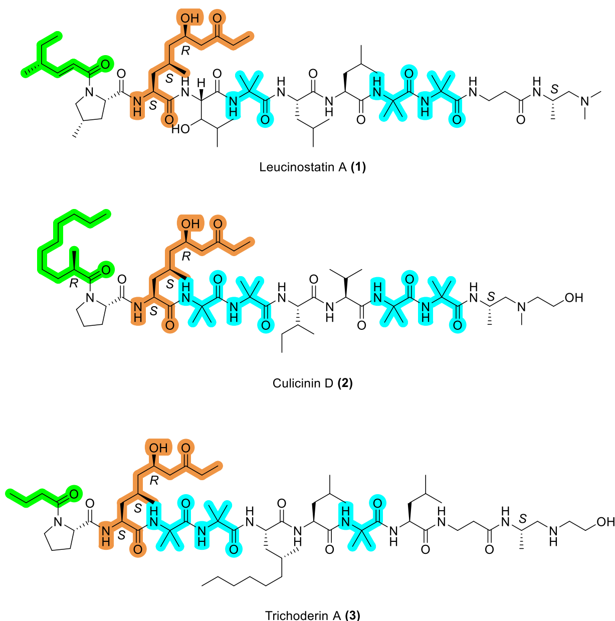
Figure 2. Comparative chemical structure of the AHMOD-containing aminolipopeptides leucinostatin A (1), culicinin D (2), and trichoderin A (3). Shared motifs are highlighted accordingly in color: N-terminus lipid tail (green), AHMOD (orange), Aib (blue).
