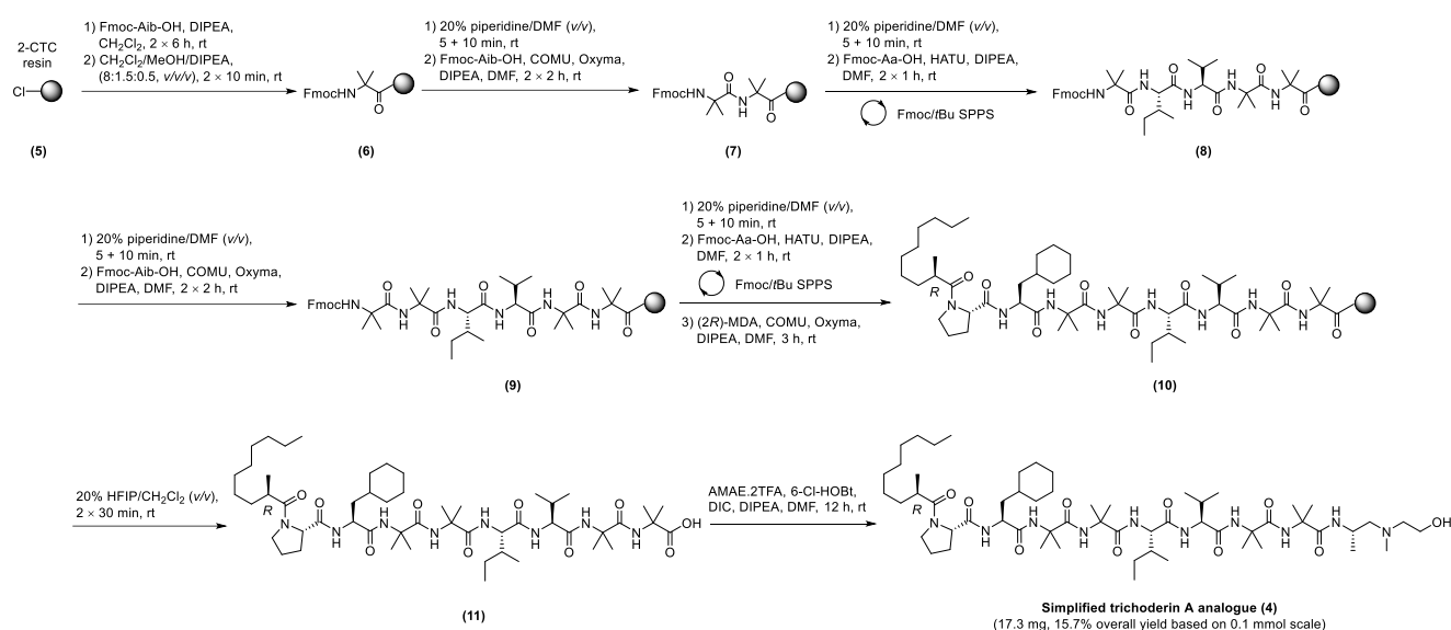
Scheme 1. Hybrid solid-/solution-phase synthesis of the simplified trichoderin A analogue (4).
