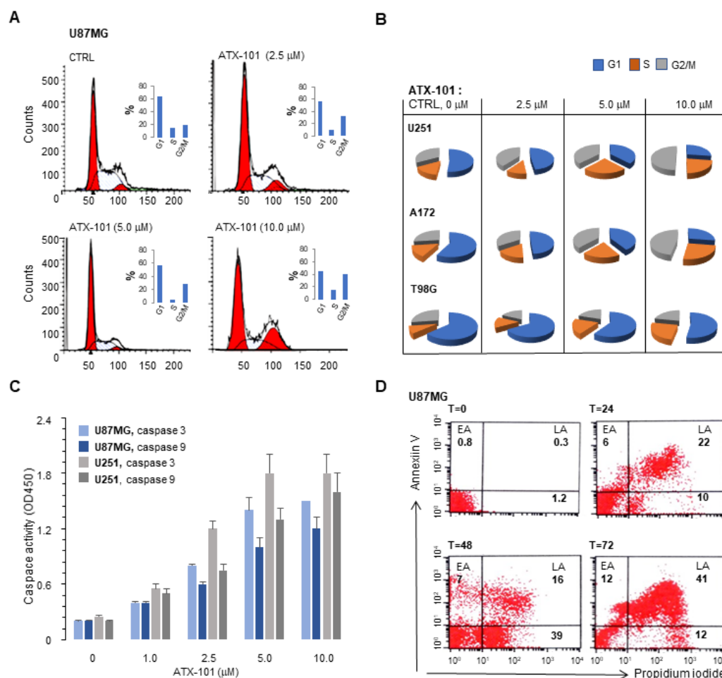
Figure 3. ATX-101 induces G2/M cell arrest and mediates apoptosis. (A) Cell cycle analysis of U87MG cells after treatment with ATX-101 (2.5–10 \mu M) for 24 h. Diploid G1 and diploid G2 cells are marked in red. (B) Graphic presentations of cell cycle analysis as in A for U251, A172, and T98G cells. (C) Enzymatic caspase 9 and 3 activity in U87MG and U251 cells treated with ATX-101 (2.5–10 \mu M) for 24 h. Means \pm SD of three independent experiments analyzed in triplicates. (D) Annexin V and necrosis (by propidium iodide) FACS analyses of U87MG at different time points (T = hours) after addition of 2.5 \mu M ATX-101. EA = early apoptosis. LA = late apoptosis.
