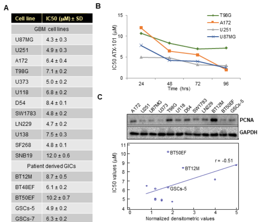
Figure 1. ATX-101 inhibits cell proliferation of GBM and GICs cells in vitro. (A) Twelve GBM cell lines and 5 GICs were examined for viability after treatment with ATX-101 (0.1–10 \mu\text{M} ). For the five GICs cell lines, the evaluation of cell proliferation was made by using sphere formation assay at clonal growth analyzed after 21 days. IC50 values are calculated for 12 GBM cell lines and 5 GICs at 72 h. (B) IC50 values for ATX-101 determined for 4 GBM cell lines over 96 h. (C) Upper panel: Western blots showing PCNA and GAPDH expression levels in 9 GBM and 3 GICs cell lines. Uncropped Western blots are shown in Supplementary Figure S2. In the lower panel, PCNA levels normalized against GAPDH were plotted against IC50s. GICs are marked in the graph and the r value ( -0.51 ) is depicted in the graph.
