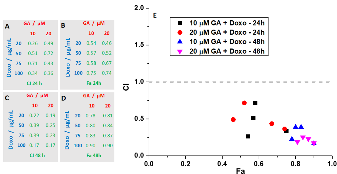
Figure 6. Effects of combination therapy of GA and Doxo on HT-29 spheroids. (A,C) Combination index (CI) values at the concentrations tested. (B,D) Fraction affected (Fa) values at the concentrations tested. (E) The CI versus Fa values, plotted for different conditions, indicate synergism for all tested conditions. CI < 1 indicates synergism, CI = 1 additivity, whereas CI > 1 indicates antagonism.
