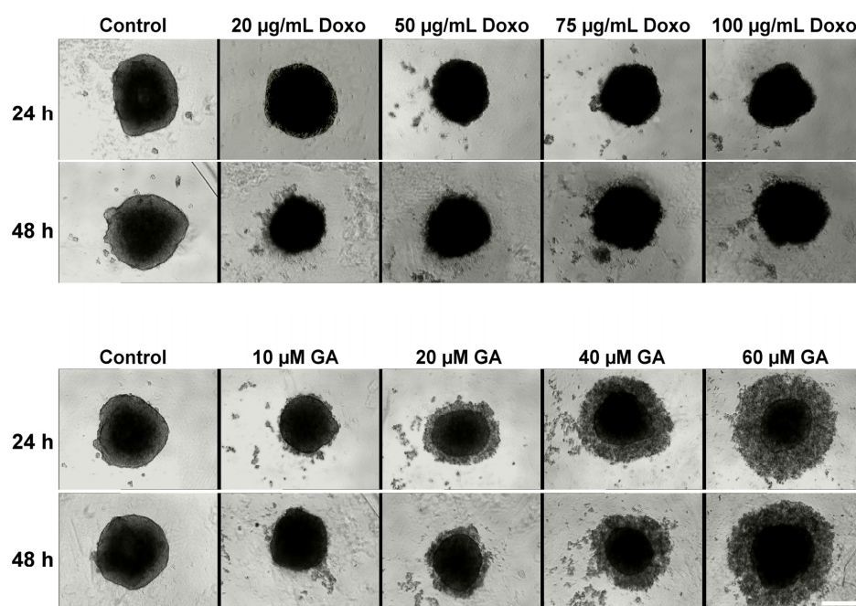
Figure 2. Cytotoxic effects of doxorubicin (Doxo) and gramicidin A (GA) on HT-29 spheroids. Spheroids were obtained after seeding 5000 cells/well and were grown for three days. On the third day of spheroid growth, different concentrations of Doxo (20, 50, 75, and 100 \mu g/mL) and GA (10, 20, 40, and 60 \mu M) were added and the effects were monitored through transmission microscopy at 24 and 48 h. The scale bar is 200 \mu m and is the same for all images.
