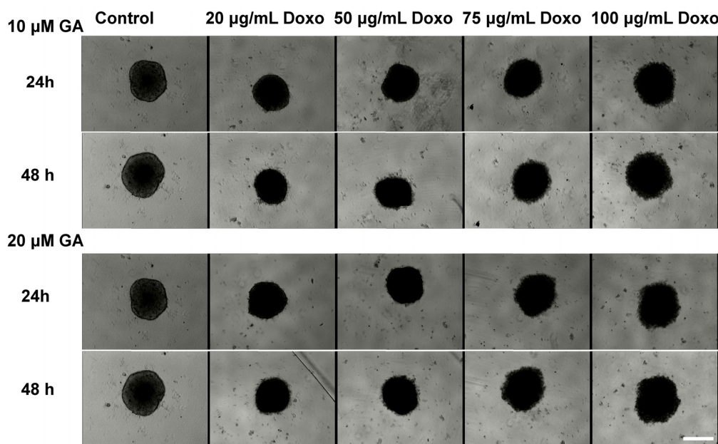
Figure 3. Cytotoxic effects of Doxo in combination with GA on HT-29 spheroids. Spheroids were obtained after seeding 5000 cells/well and were grown for three days. On the third day of spheroid growth, different concentrations of Doxo (20, 50, 75, and 100 \mu\text{g/mL} ) and GA (10, 20, 40, and 60 \mu\text{M} ) were added and the effects were monitored through transmission microscopy at 24 and 48 h. The scale bar is 200 \mu\text{m} and is the same for all images.
