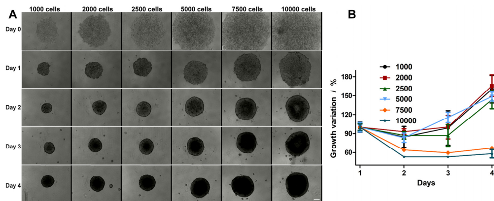
Figure 1. (A) Spheroid evolution monitored over 5 days at different seeding densities (1000, 2000, 2500, 5000, 7500, and 10,000 cells/well). (B) Growth kinetics of HT-29 spheroids. The scale bar is 100 \mu m and is the same for all images.
