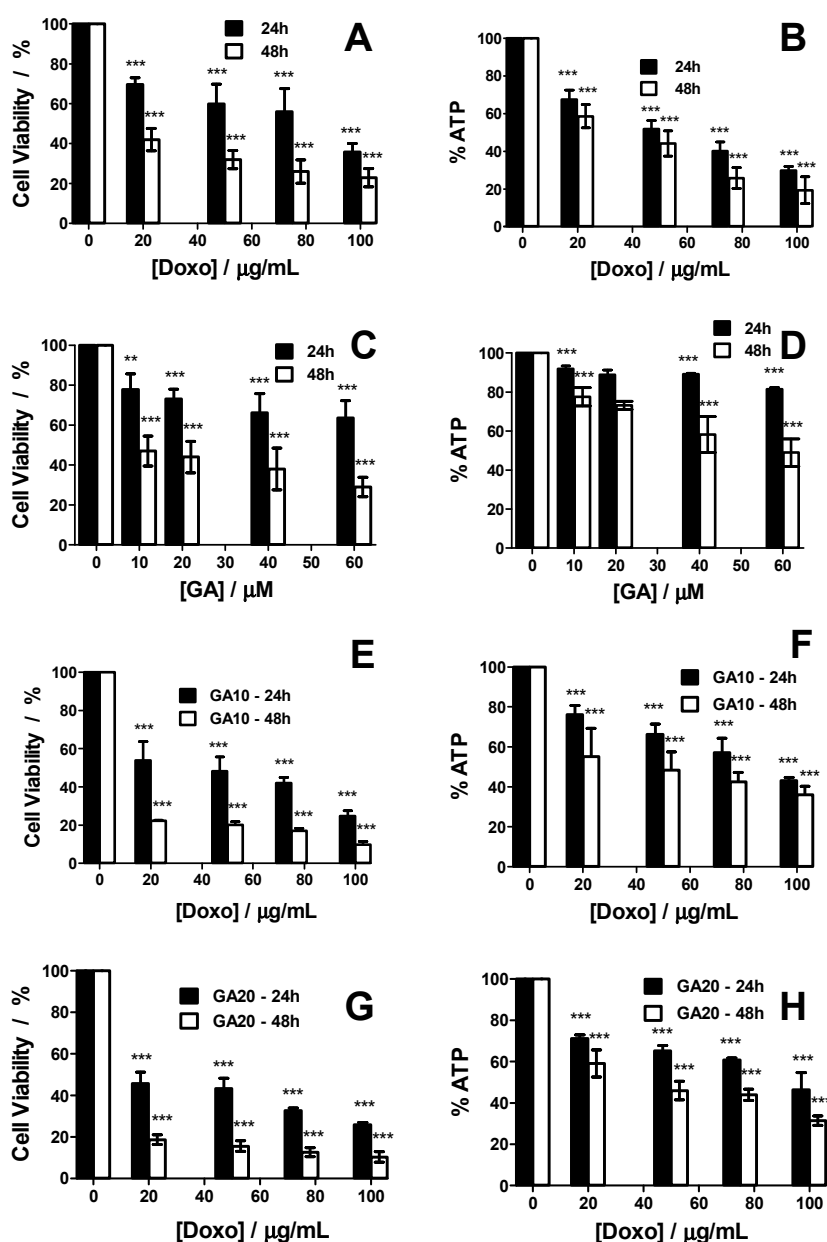
Figure 5. Cell viability of HT-29 spheroids treated with Doxo (A), GA (C), and their combination (E,G) at 24 and 48 h with increasing concentrations. ATP levels of HT-29 spheroids treated with Doxo (B), GA (D), and their combination (F,H) at 24 and 48 h with increasing concentrations. p values based on ANOVA analysis with Bonferroni's comparison post-test versus control condition. Note: ** p < 0.01 , *** p < 0.001 .
