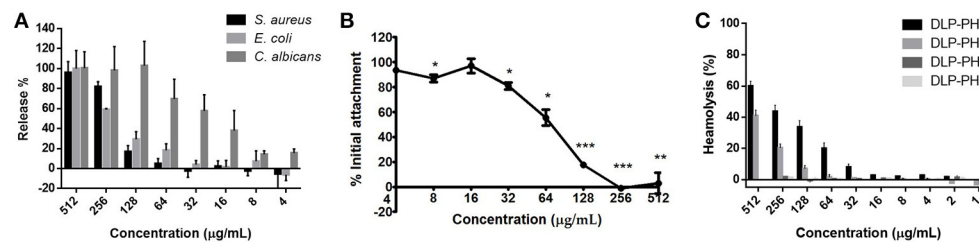
FIGURE 3 | (A) Effect of DLP-PH on cytoplasmic material release of S. aureus , E. coli , and C. albicans at 260 nm. The error bar represents the standard error for three repeats (ANOVA, P < 0.05 ). (B) Effect of DLP-PH on the P. aeruginosa biofilm initial attachment. The error bar represents the standard error for three repeats. The significance is given as * p < 0.05 ; ** p < 0.01 ; *** p < 0.001 . (C) Relative haemolysis of DLP-PH and its deviates on horse red blood cells. The 100% haemolysis was defined using haemolytic effect induced by 1% Triton X-100 (ANOVA, P < 0.05 ).
